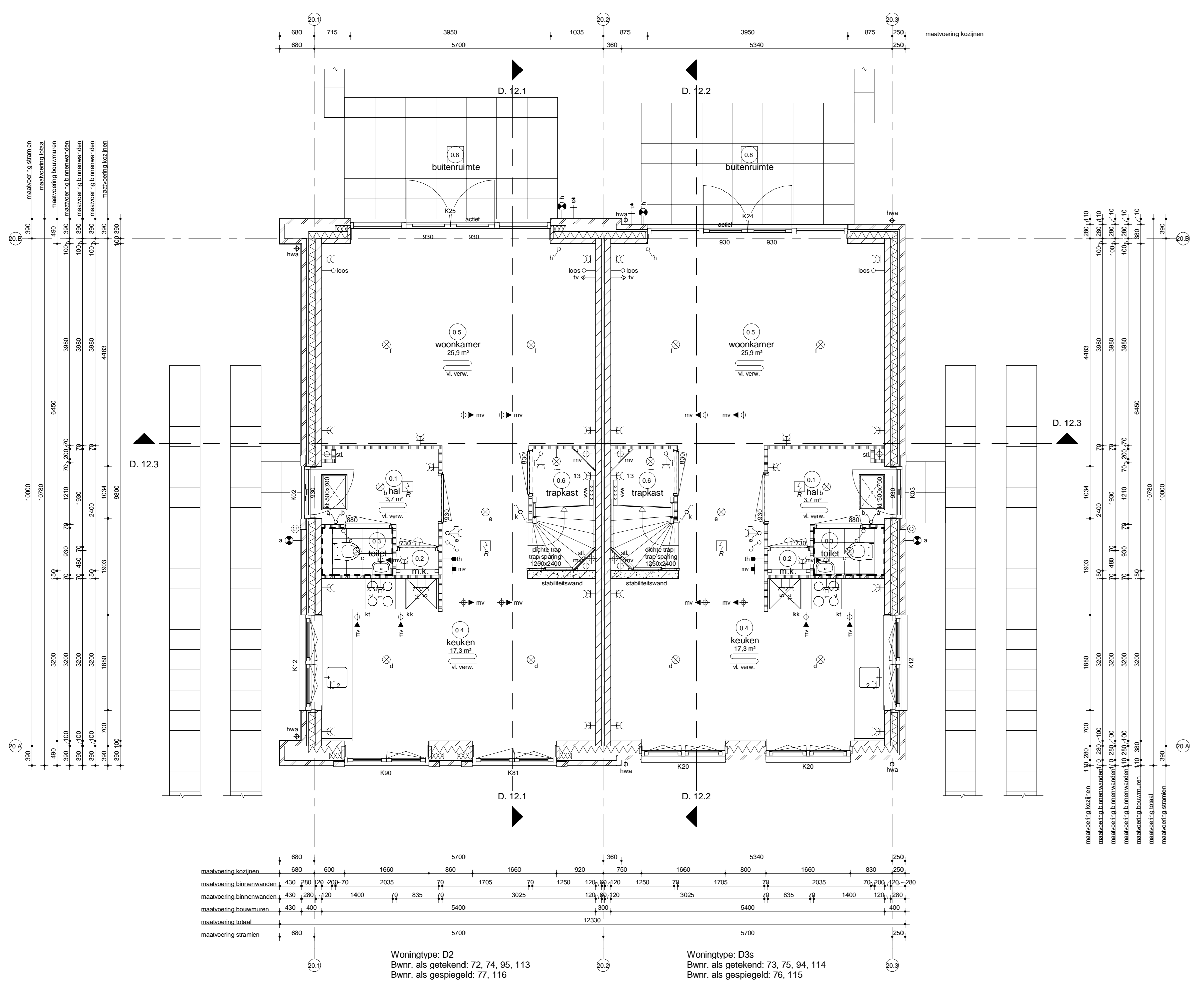
Begane grond bk. vloer = peil = 0 blok 20, 29 & 35
